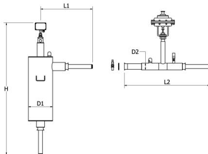
Electronic Cryovent
