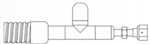
Cryochiller conn, Female seal-lok 1/2" or 1/4" HVCR
